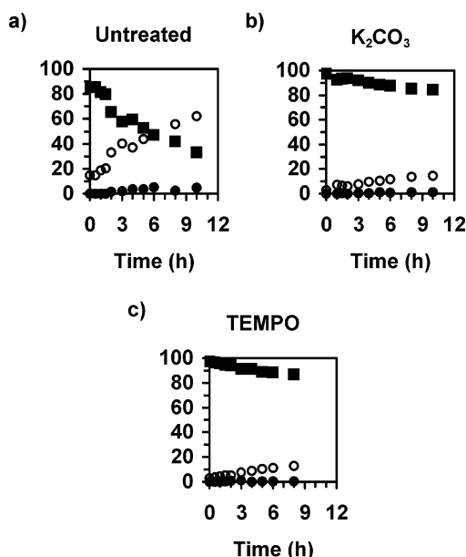
Figure 3. Plots of the mole percentage of alkene residues ( F_{a.r.} \times 100\% ) attributed to PPA (■), cyclohexadiene moieties (○), and extruded 1,3,5-C 6 H 3 Ph 3 (●) for solutions in (a) CDCl 3 , (b) CDCl 3 pretreated with K 2 CO 3 , and (c) CDCl 3 containing 33 mol % TEMPO thermally treated at 60 °C. Thermal treatments were performed on degassed samples in NMR sample tubes sealed under vacuum. Heating was performed in the NMR spectrometer.
